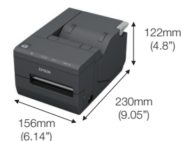
TM-L500A without LCD
