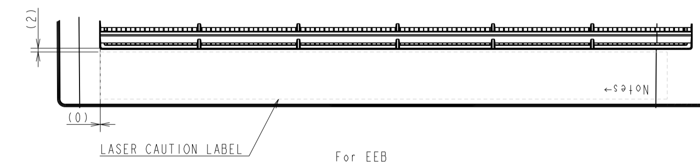
Detail A Scale 1:2
